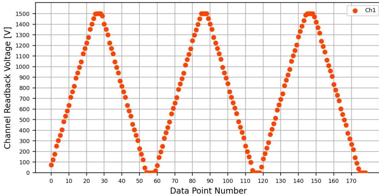
Voltage Ramp Test (Python) Bd #070, Slot #10, Ch #1
