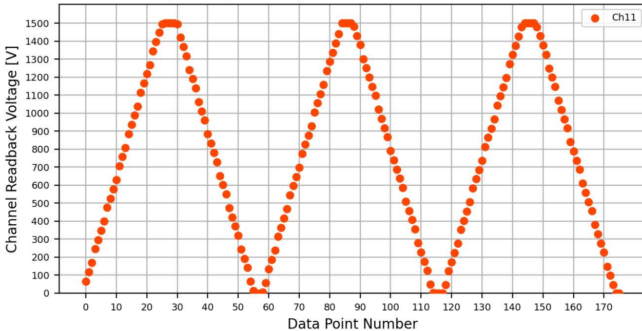
Voltage Ramp Test (Python) Bd #070, Slot #10, Ch #11
