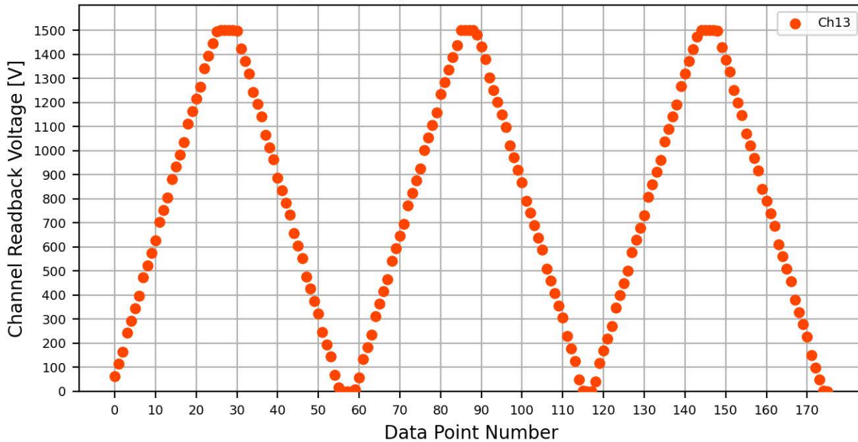
Voltage Ramp Test (Python) Bd #070, Slot #10, Ch #13
