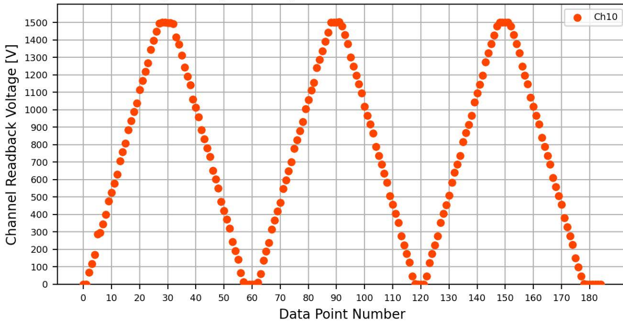
Voltage Ramp Test (Python) Bd #070, Slot #10, Ch #10
