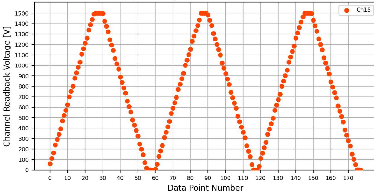
Voltage Ramp Test (Python) Bd #070, Slot #10, Ch #15
