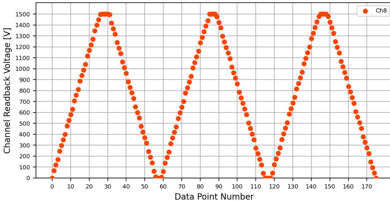
Voltage Ramp Test (Python) Bd #070, Slot #10, Ch #8
