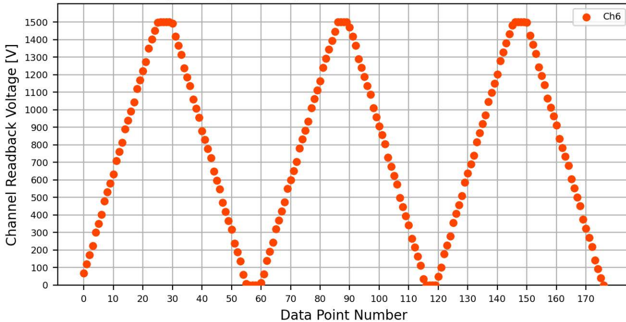
Voltage Ramp Test (Python) Bd #070, Slot #10, Ch #6
