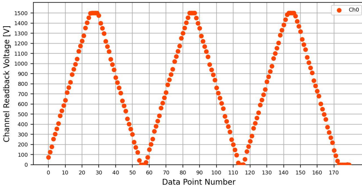
Voltage Ramp Test (Python) Bd #070, Slot #10, Ch #0
