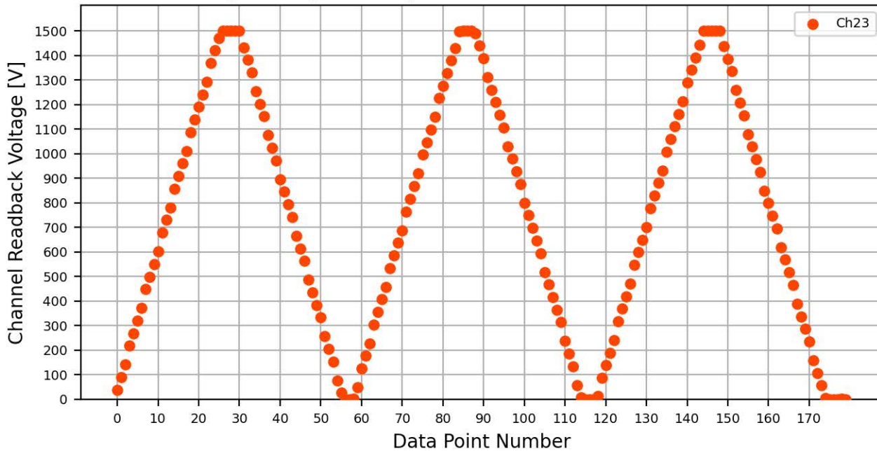
Voltage Ramp Test (Python) Bd #070, Slot #10, Ch #23
