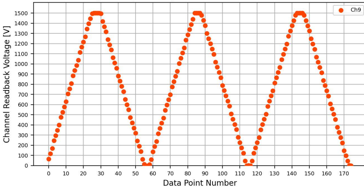
Voltage Ramp Test (Python) Bd #070, Slot #10, Ch #9
