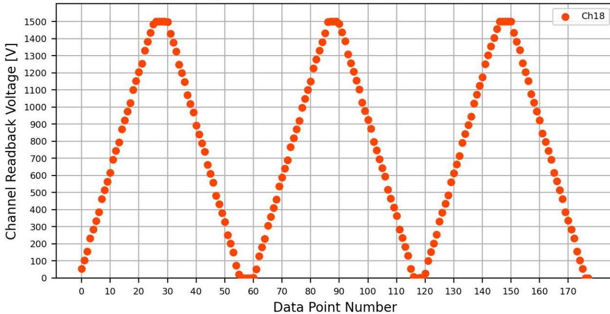
Voltage Ramp Test (Python) Bd #070, Slot #10, Ch #18
