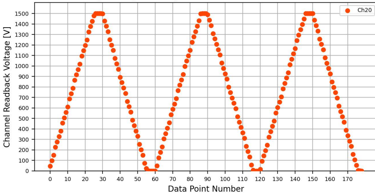
Voltage Ramp Test (Python) Bd #070, Slot #10, Ch #20
