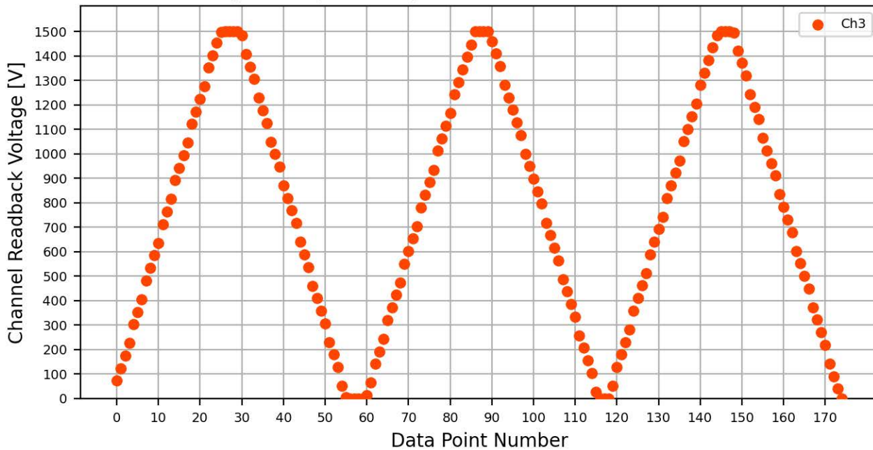
Voltage Ramp Test (Python) Bd #070, Slot #10, Ch #3
