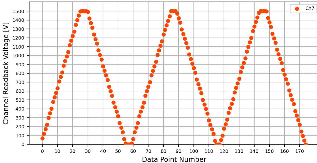
Voltage Ramp Test (Python) Bd #070, Slot #10, Ch #7
