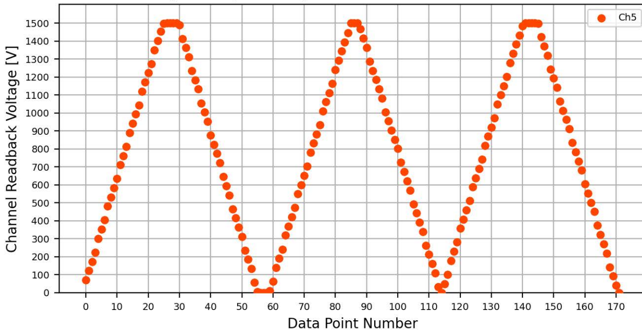
Voltage Ramp Test (Python) Bd #070, Slot #10, Ch #5
