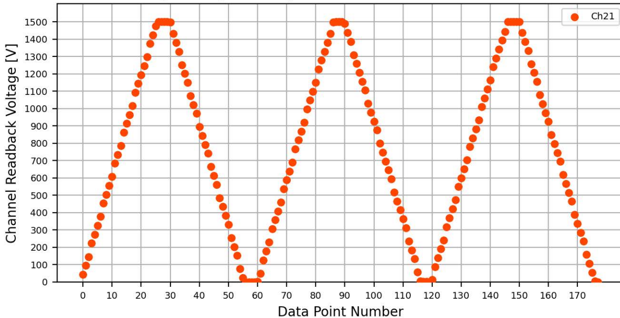
Voltage Ramp Test (Python) Bd #070, Slot #10, Ch #21
