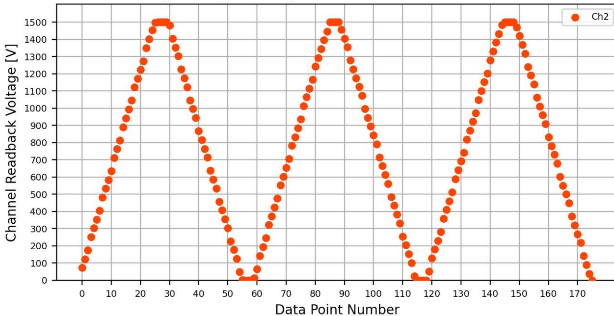
Voltage Ramp Test (Python) Bd #070, Slot #10, Ch #2
