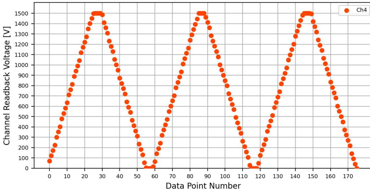
Voltage Ramp Test (Python) Bd #070, Slot #10, Ch #4
