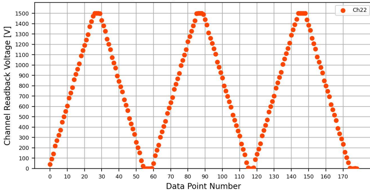
Voltage Ramp Test (Python) Bd #070, Slot #10, Ch #22
